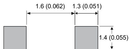
SOD-123FL
