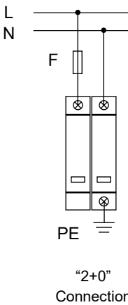
Single phase system
