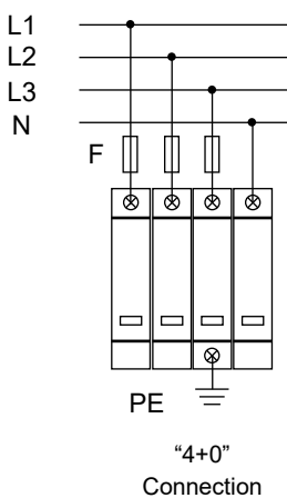
Three phase system
